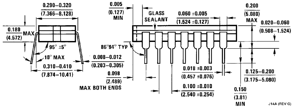
14-Lead Ceramic Dual-In-Line Package (J) Order Number DM54LS26J NS Package Number J14A
