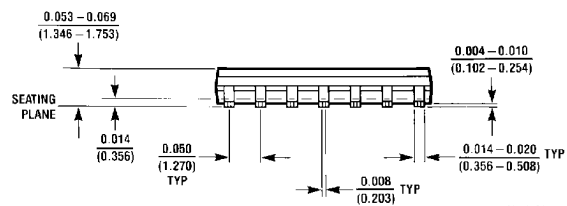
14-Lead Small Outline Molded Package (M) Order Number DM74LS26M NS Package Number M14A
